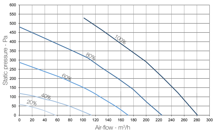
Intake curve according to Reg.1253/2014 (ErP).
